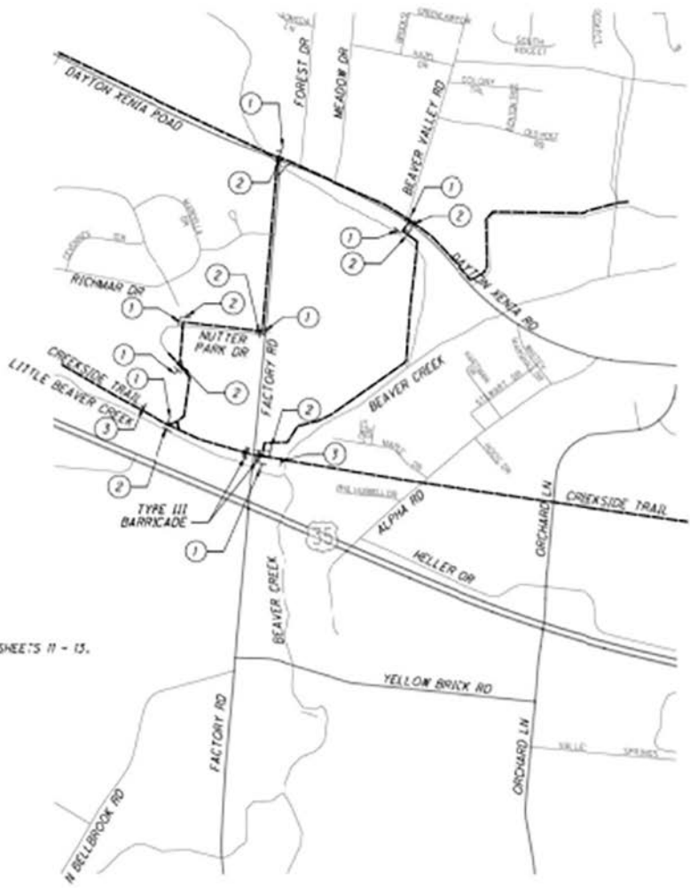
DETOUR SIGNING
